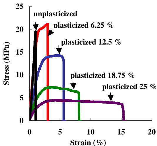
Figure 1. Effect glycerol and polyethylene glycol as plasticizer mix on the tensile properties of zein films.
