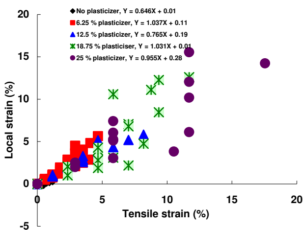
Figure 3. Relationship between overall tensile (grip to grip separation) and local strain (fluospheres® distances)
