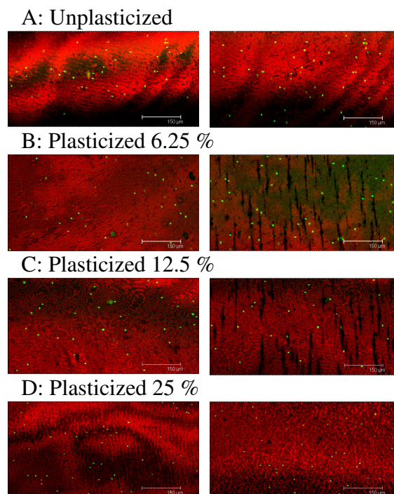
Figure 2. CLSM micrographs of unplastified and plasticized zein films at different strain
