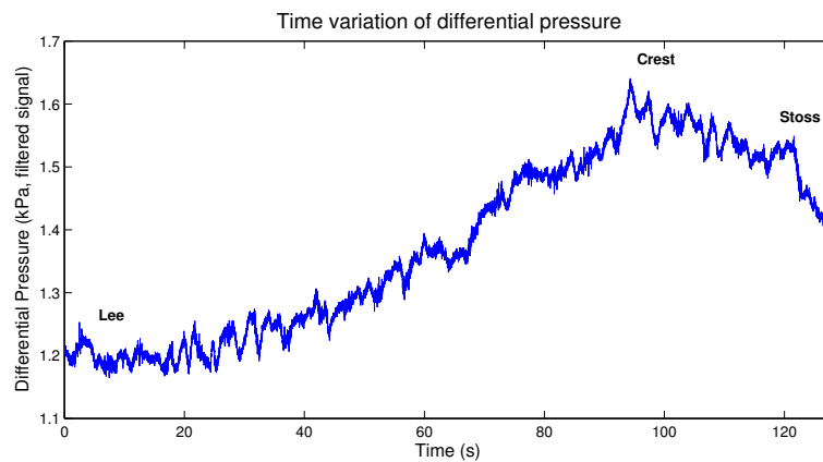
Figure 7: Fluid pressure on the crest, at the lee and on the stoss. U \approx 0.27 m/s.
